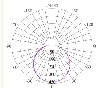
Photometric Diagram
